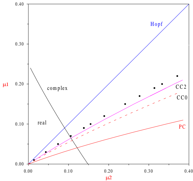
Fig. 2. The (\mu_2, \mu_1) parameter space of Eq. (4) shows the eigenvalues at the origin, the locus of the Hopf bifurcation from B and the principal homoclinic bifurcation criteria. The dotted curve corresponds to the numerical values, (PC) corresponds to the period criterion given in Eq. (35), (CC0) is the collision criterion given in Eq. (34) and (CC2) is the collision criterion using the second order of x(t) given in Eq. (25).
